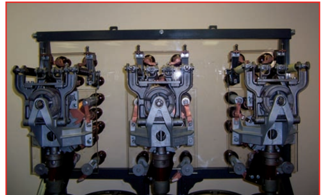
GE LR-83 Load Tap Changer Training Model
