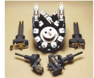
FPE Tap Head and Switches
