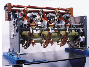
Converted GE LRT200-2 Load Tap Changer
