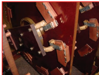
TLH-21 Moveable Contacts in a Bridging Position
