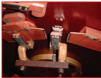
TLH-21 Moveable and Stationary Contacts
